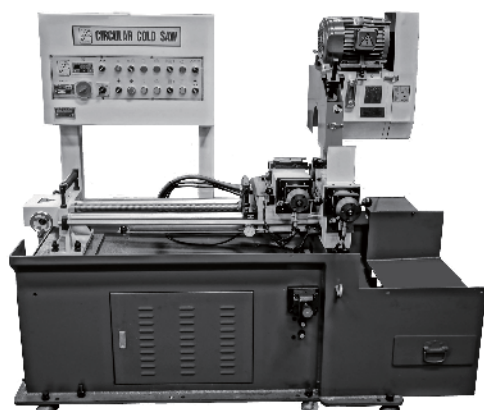
Circular Cold Sawing Machine
